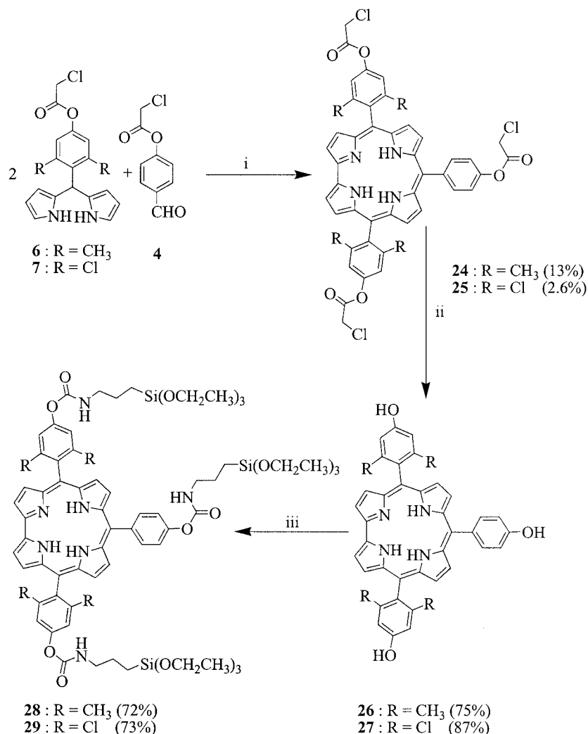
Scheme 7. i) 1: TFA, CH 2 Cl 2 ; 2: DDQ. ii) PhCH 2 NH 2 , THF, EtOH. iii) IPTES (12 equiv.), i Pr 2 NEt (6 equiv.), THF, MeCN, 7 days.
